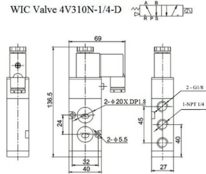
WIC Valve 4V310N-1/4-D
